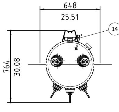
GROUNDING COUNECTOR DETAIL
